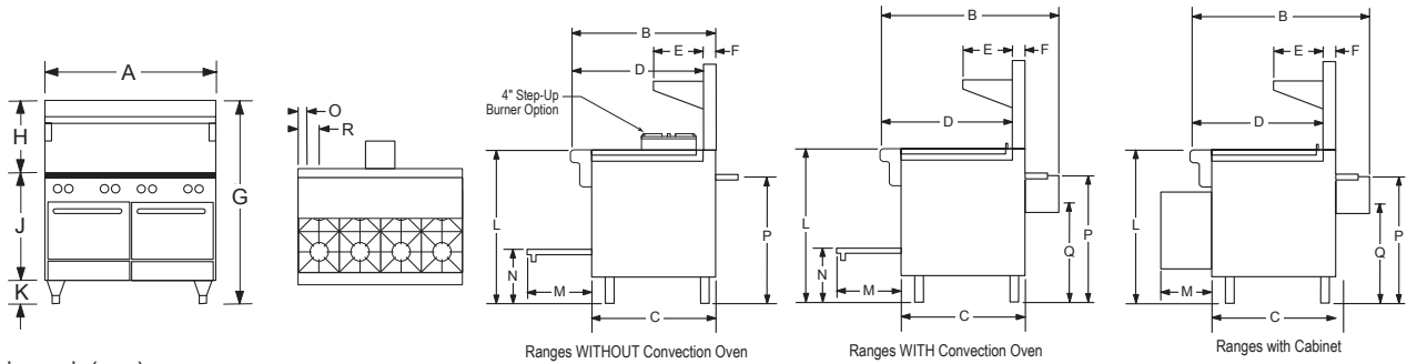
Dimensions - in(mm)
